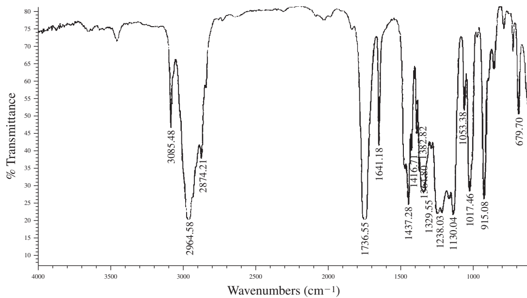
Infrared spectrum
