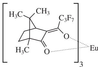
Tris[3-(heptafluoropropylhydroxymethylene)- d -camphorato] europium(III) [ \text{Eu}(\text{hfc})_3 ]
