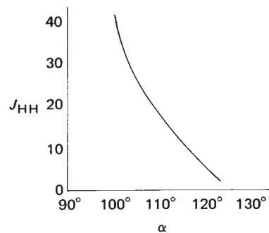
FIGURE 7.4 The dependence of the magnitude of {}^2J_{\text{HCH}} , the geminal coupling constant, on the HCH bond angle \alpha .
