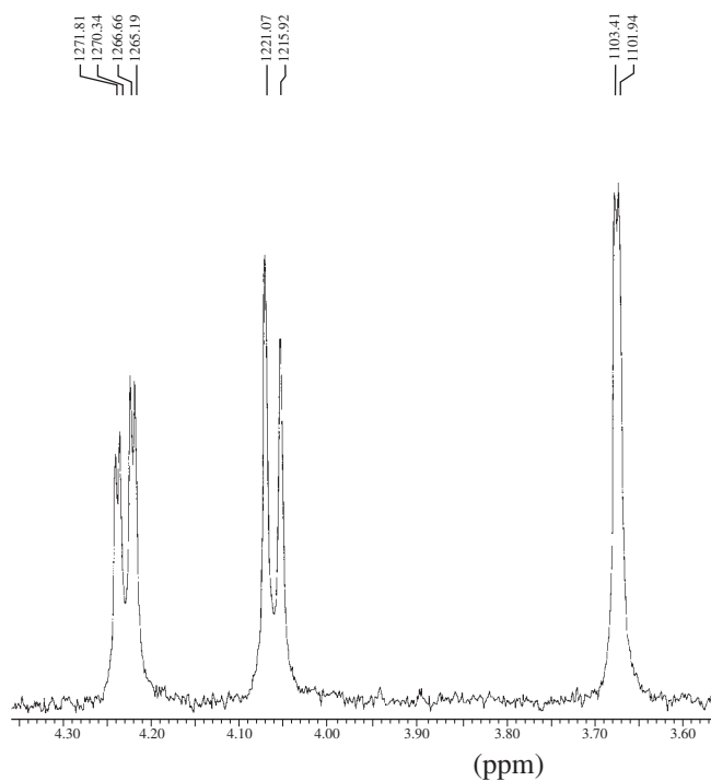
Spectrum A
