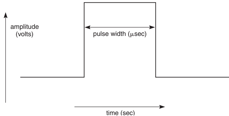
FIGURE 9.5 A square-wave pulse.
