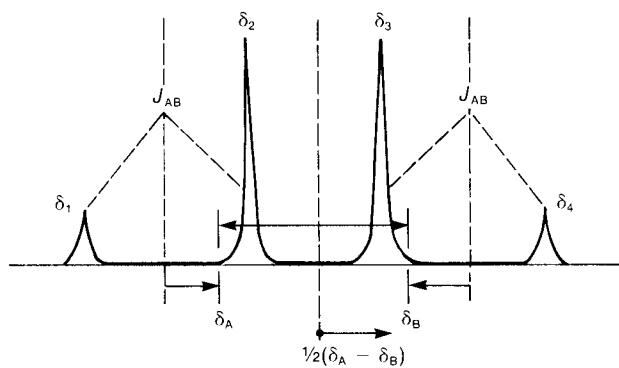
FIGURE 7.42 The relationships among the chemical shifts, line positions, and coupling constant in a two-proton AB system that exhibits second-order effects.
