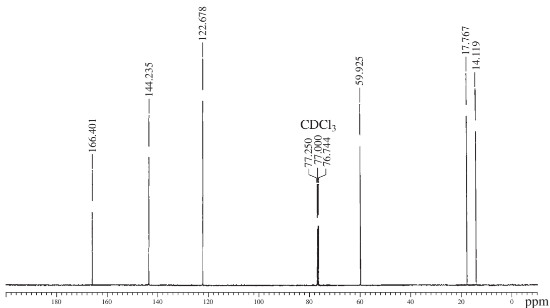
FIGURE 9.22 ^{13}\text{C} NMR spectrum for \text{C}_6\text{H}_{10}\text{O}_2 .
