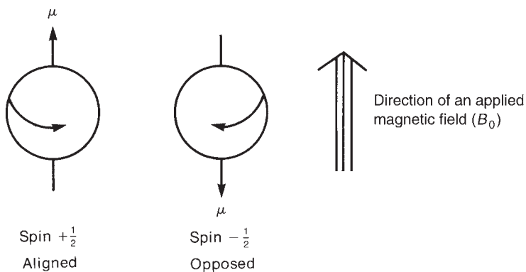
FIGURE 5.1 The two allowed spin states for a proton.
