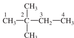
2,2-Dimethylbutane
