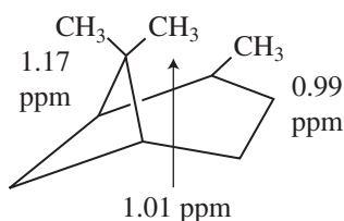
Pinane
