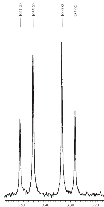
Spectrum B
