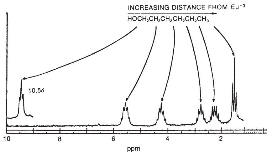
FIGURE 8.22 The 100-MHz NMR spectrum of 1-hexanol with 0.29-mole equivalent of \text{Eu}(\text{dpm})_3 added. (From Sanders, J. K. M., and D. H. Williams, Chemical Communications (1970): 442. Reprinted by permission.)
