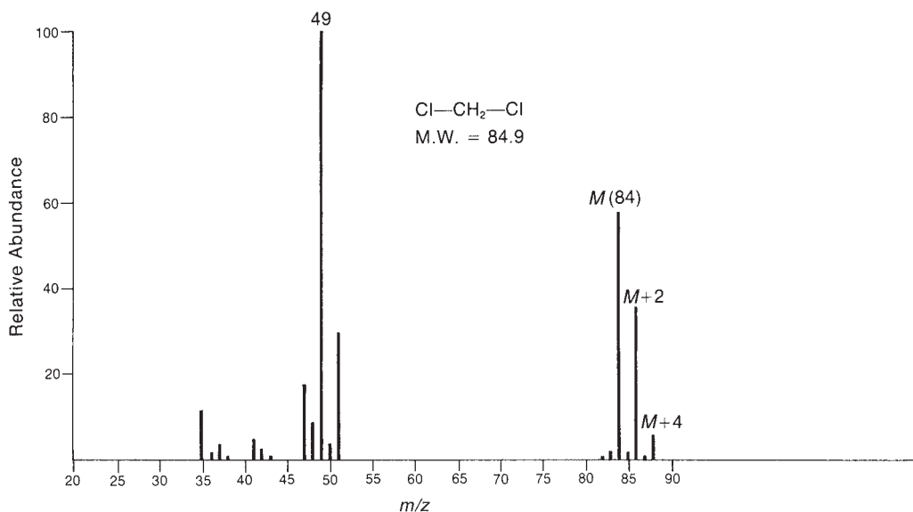
FIGURE 4.67 Mass spectrum of dichloromethane.
