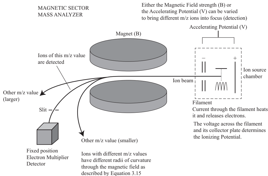
FIGURE 3.11 Schematic of a magnetic sector mass analyzer.
