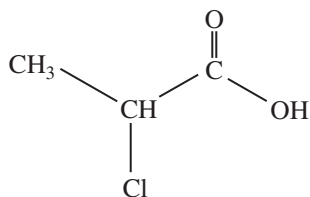
2-chloropropanoic acid
