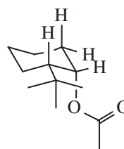
lowest energy conformer for cis diastereomer
