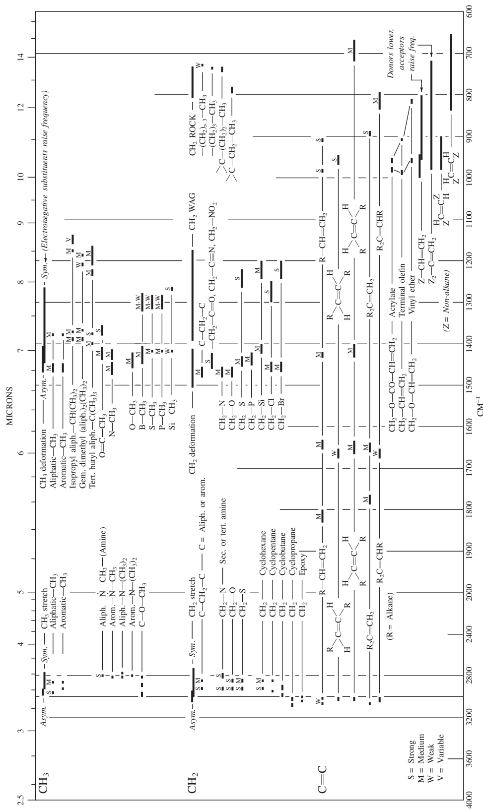
Colthup spectra-structure correlation charts for infrared frequencies in the 4000-600 \text{cm}^{-1} region from Lin-Vien, D., N. B. Colthup, W. G. Fateley, and J. G. Grasselli, The Handbook of Infrared and Raman Characteristic Frequencies of Organic Molecules , Academic Press, New York, 1991.
