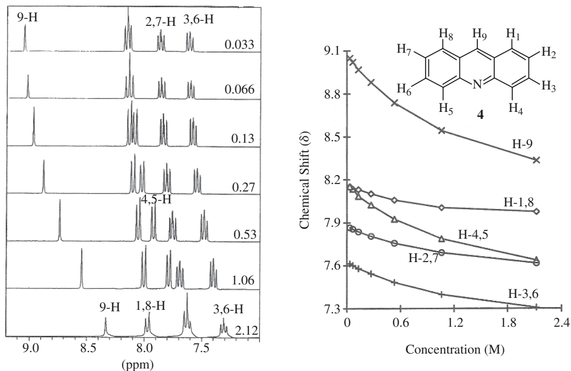
FIGURE 8.18 1 H NMR spectra of acridine in CD 3 OD at different concentrations (mol/L). (From Mitra, A., P. J. Seaton, R. A. Assapour, T. Williamson; Tetrahedron 54 (1998): 15489–15498.)
