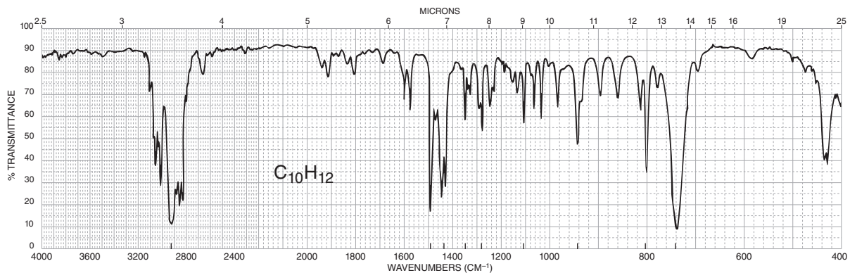
(g) C_{10}H_{12} (two six-membered rings)
