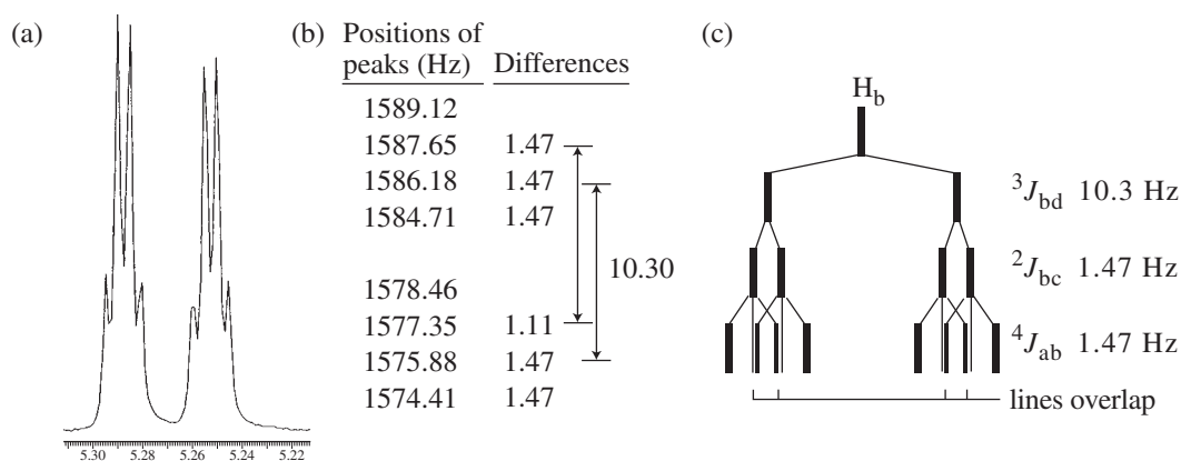
FIGURE 7.56 Allyloxyanisole. (a) Expansion of H_b . (b) Peak positions (Hz) and selected frequency differences. (c) Splitting tree diagram showing the origin of the splitting pattern.
