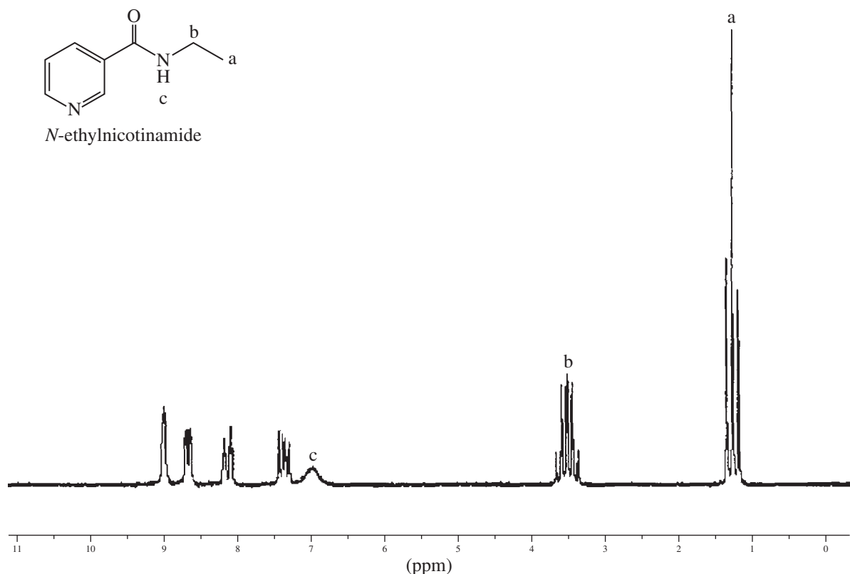
FIGURE 8.14 ^1\text{H} NMR spectrum of N -ethylnicotinamide.
