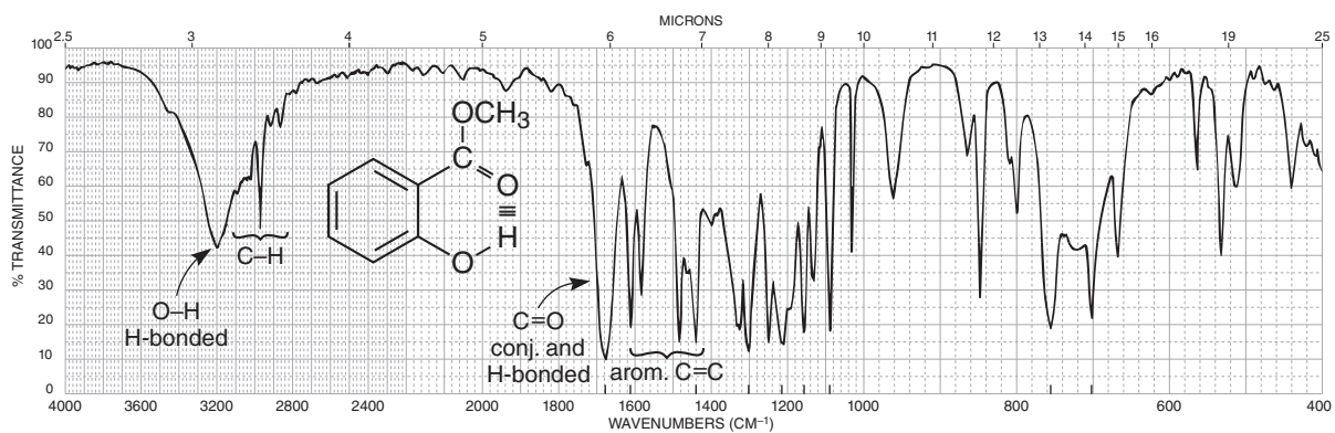
FIGURE 2.51 The infrared spectrum of methyl salicylate (neat liquid, KBr plates).
