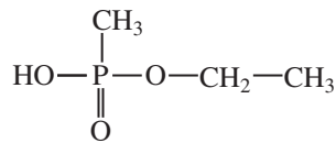
Ethyl methylphosphonate
