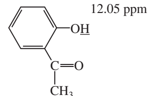
o -Hydroxyacetophenone
