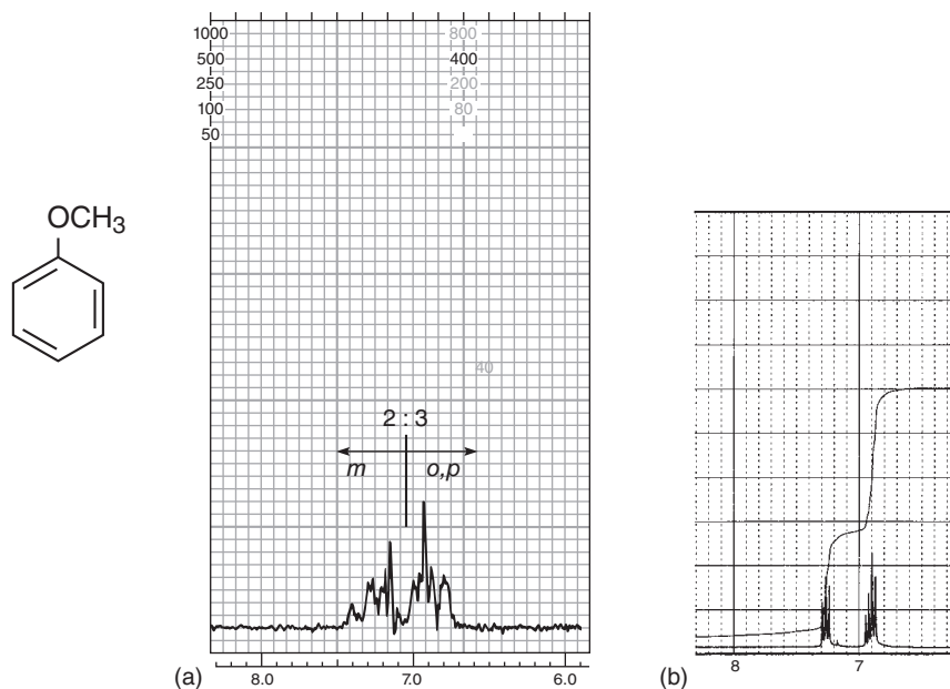
FIGURE 7.60 The aromatic ring portions of the ^1\text{H} NMR spectrum of anisole at (a) 60 MHz and (b) 300 MHz.
