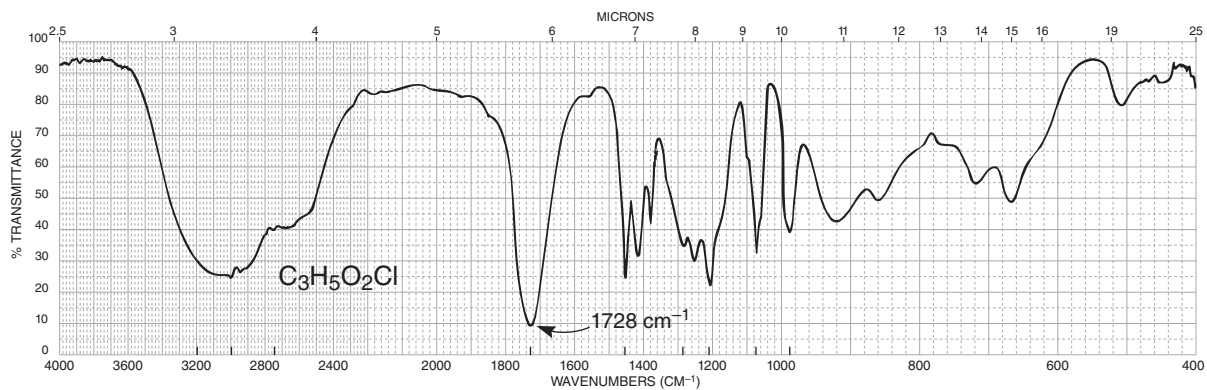
(f) C_3H_5O_2Cl
