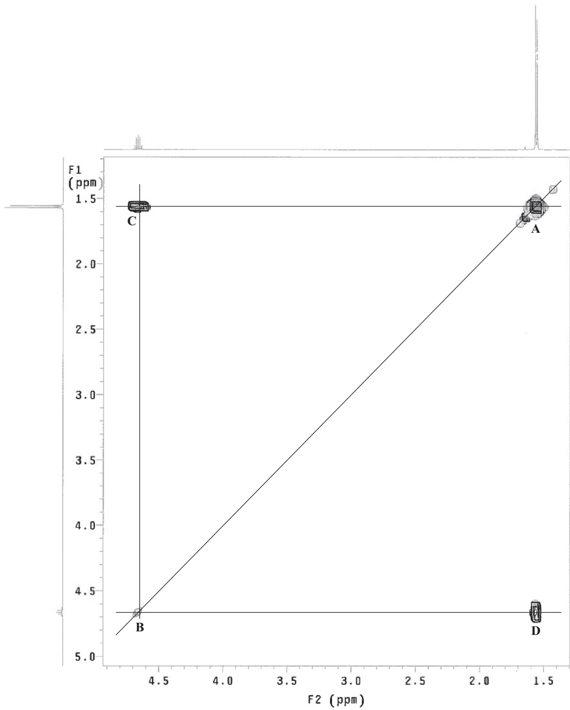
FIGURE 9.13 COSY spectrum of 2-nitropropane (125 MHz).
