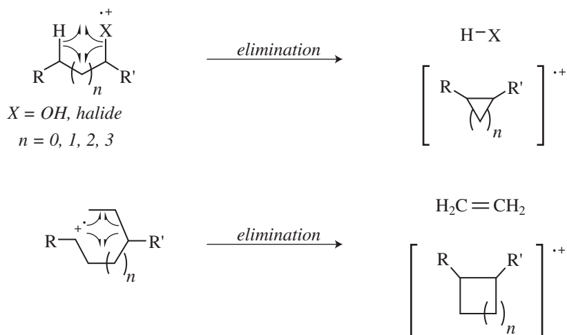
FIGURE 4.3 Common two-bond fragmentations ( X = \text{heteroatom} ).
