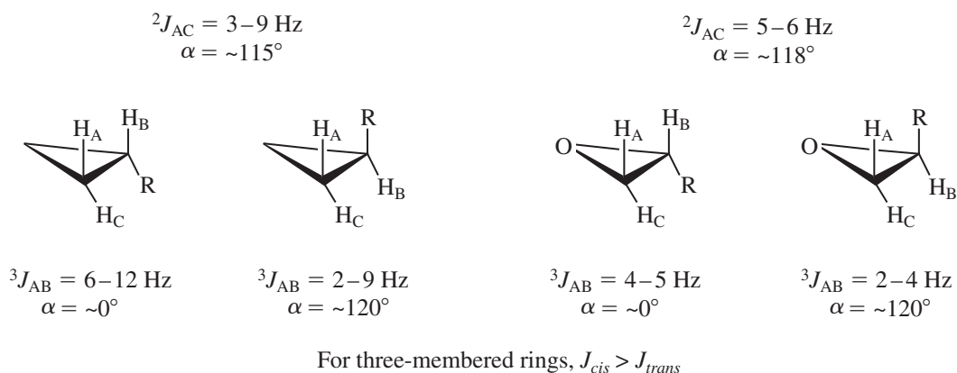
FIGURE 7.10 Vicinal couplings in three-membered ring derivatives.
