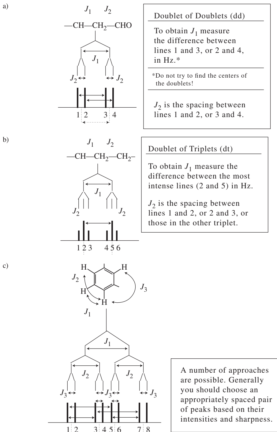
FIGURE 7.37 Determining coupling constants for a) doublet of doublets (dd), b) doublet of triplets (dt), and c) doublet of doublets of doublets (ddd) patterns.
