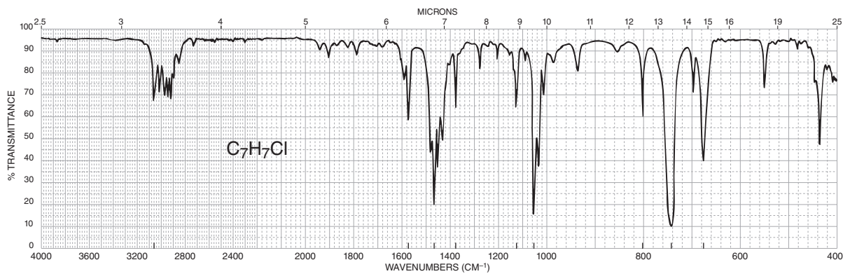
(f) C_3H_5O_2Cl
