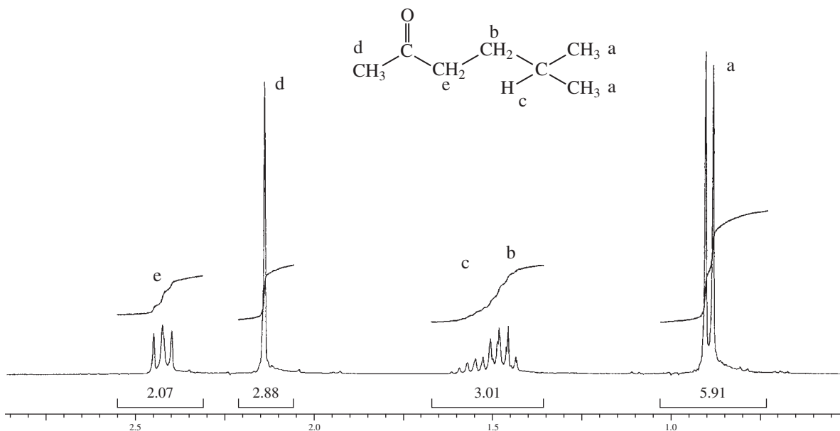
FIGURE 5.47 1 H spectrum of 5-methyl-2-hexanone (300 MHz).
