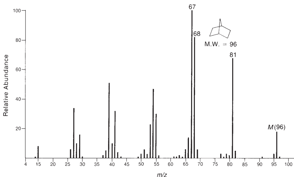
FIGURE 4.12 EI mass spectrum of bicyclo[2.2.1]heptane (norbornane).
