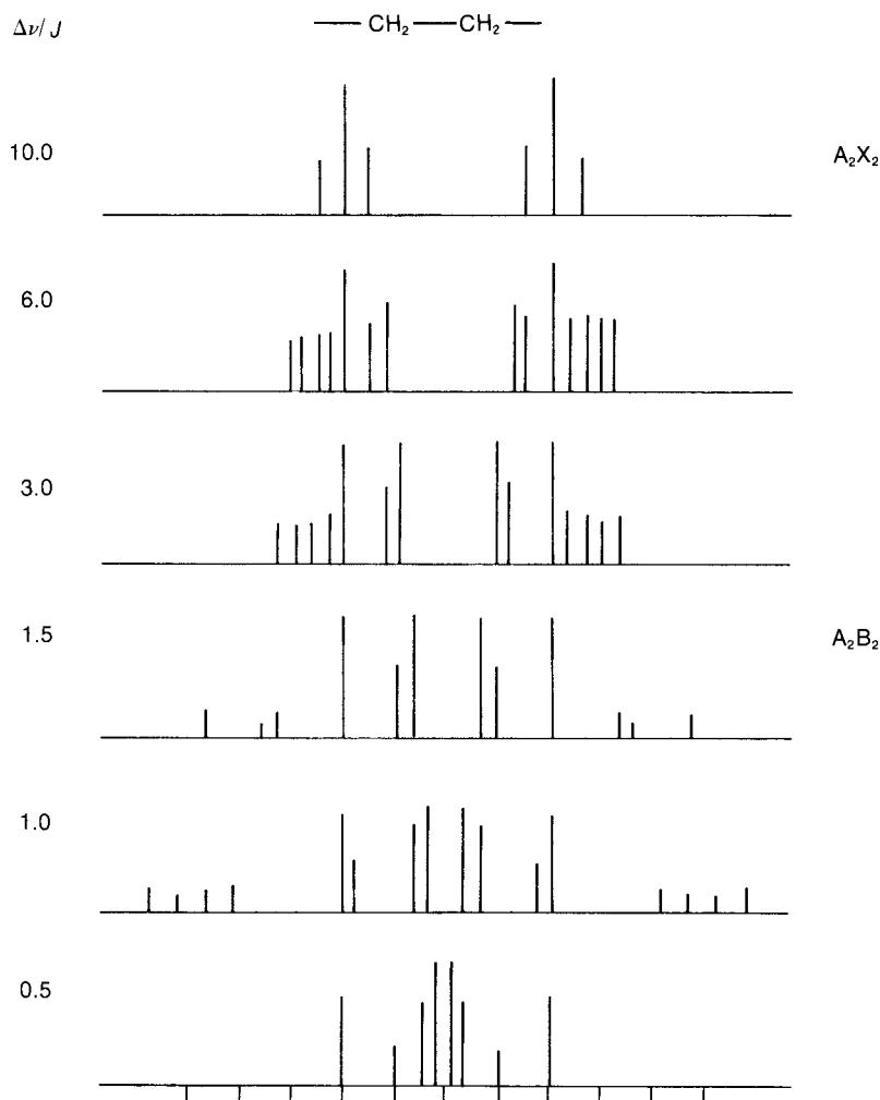
FIGURE 7.44 The splitting patterns of a four-proton system -\text{CH}_2-\text{CH}_2- for various \Delta\nu/J values.
