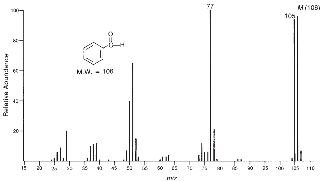
FIGURE 4.42 EI-MS of benzaldehyde.
