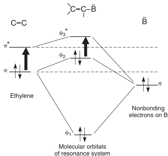
FIGURE 10.14 Energy relationships of the new molecular orbitals and the interacting \pi system and its auxochrome.
