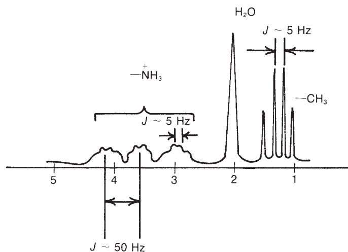
FIGURE 8.10 ^1\text{H} NMR spectrum of \text{CH}_3\text{NH}_3^+ in \text{H}_2\text{O} (pH < 1).
