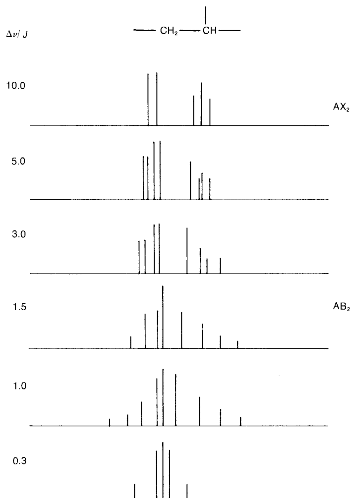
FIGURE 7.43 The splitting patterns of a three-proton system \text{---CH---CH}_2\text{---} for various \Delta\nu/J values.
