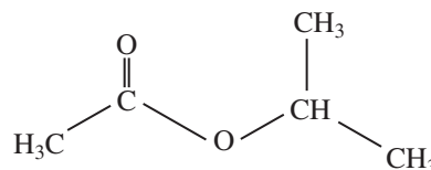
isopropyl acetate
