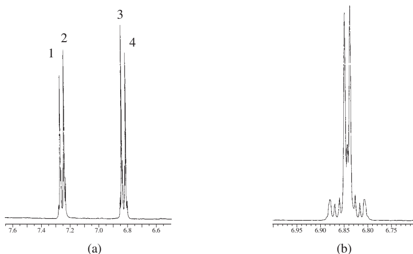
FIGURE 7.64 The aromatic ring portions of the 300-MHz ^1\text{H} NMR spectra of (a) anethole and (b) 4-allyloxyanisole.
