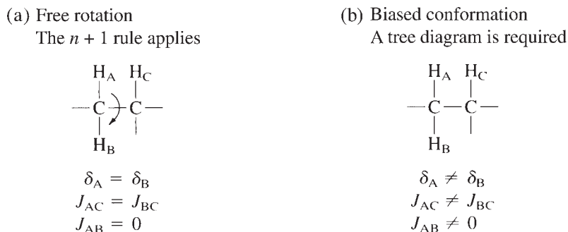
FIGURE 7.30 Two cases of splitting.
