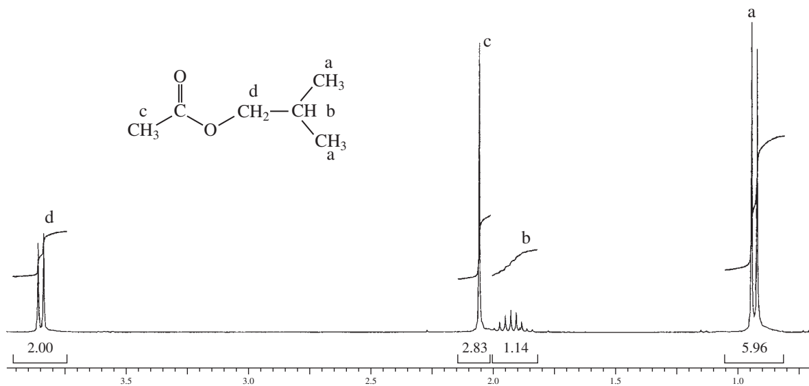
FIGURE 5.48 ^1\text{H} spectrum of isobutyl acetate (300 MHz).
