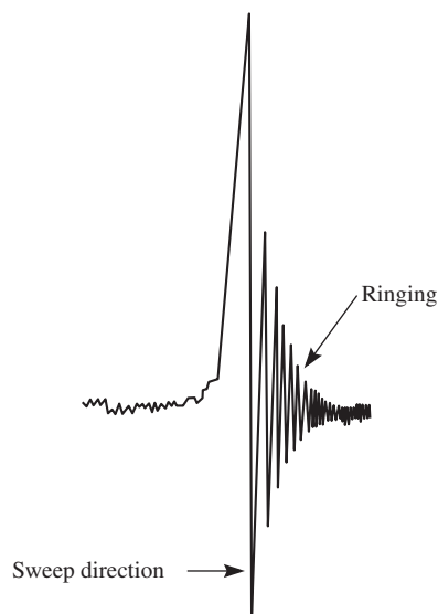
FIGURE 5.13 A CW peak that shows ringing.
