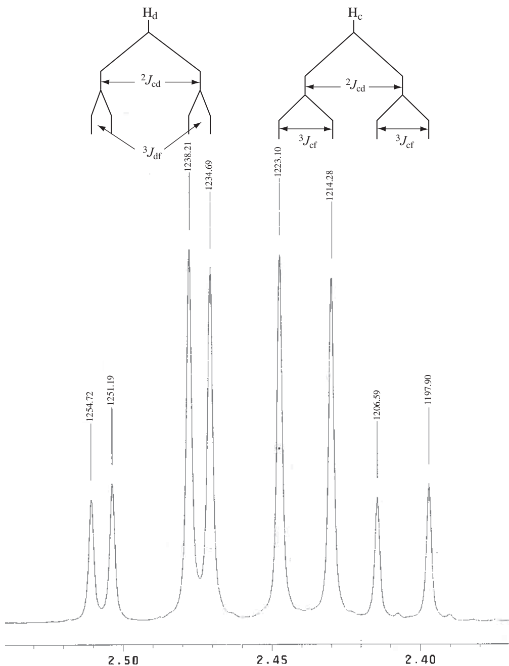
FIGURE 7.22 Expansion of the diastereotopic methylene protons in the ^1\text{H} NMR spectrum of ethyl 3-hydroxybutanoate (500 MHz, \text{CDCl}_3 ).
