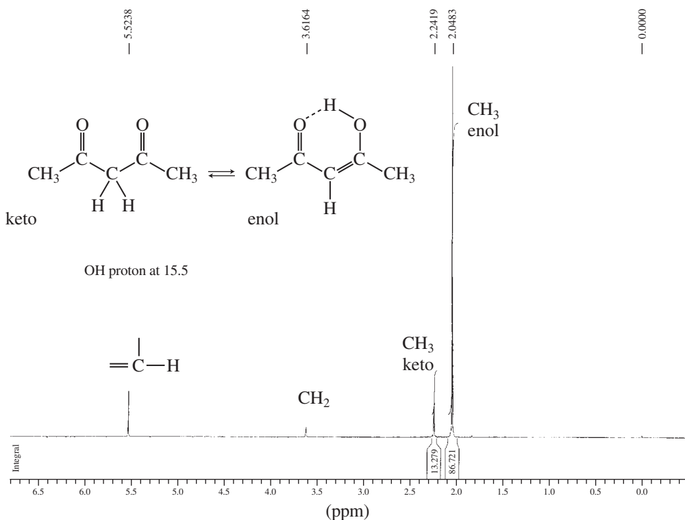
FIGURE 8.7 ^1\text{H} NMR spectrum of acetylacetone. The O–H proton of the enol tautomer is not shown.
