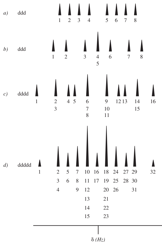
FIGURE 7.38 Numbering lines of a first-order multiplet to account for all 2^n components of the resonance. (From Hoye, T. R. and H. Zhao, Journal of Organic Chemistry 2002, 67, 4014–4016.) Reprinted by permission.
