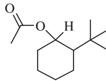
2- tert -butyl-cyclohexyl acetate
