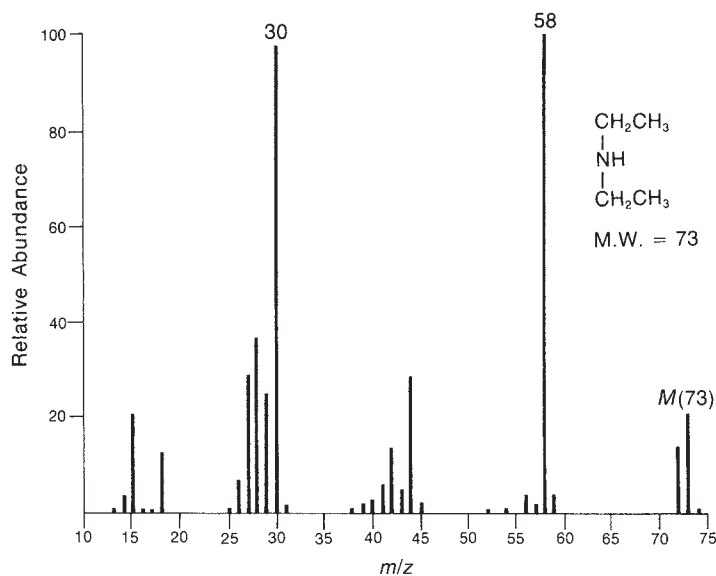
FIGURE 4.56 Mass spectrum of diethylamine.
