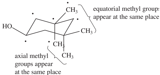
3,3,5,5-Tetramethylcyclohexanol
