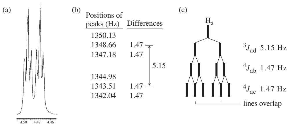
FIGURE 7.55 Allyloxyanisole. (a) Expansion of H a . (b) Peak positions (Hz) and selected frequency differences. (c) Splitting tree diagram showing the origin of the splitting pattern.
