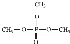
Trimethoxy phosphate
