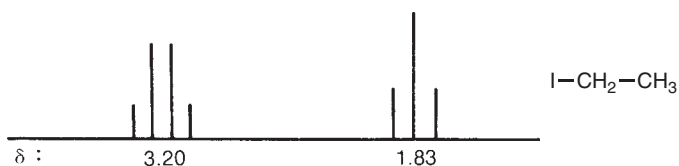
FIGURE 5.30 The ethyl splitting pattern.
