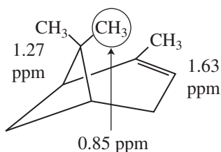
\alpha -Pinene
