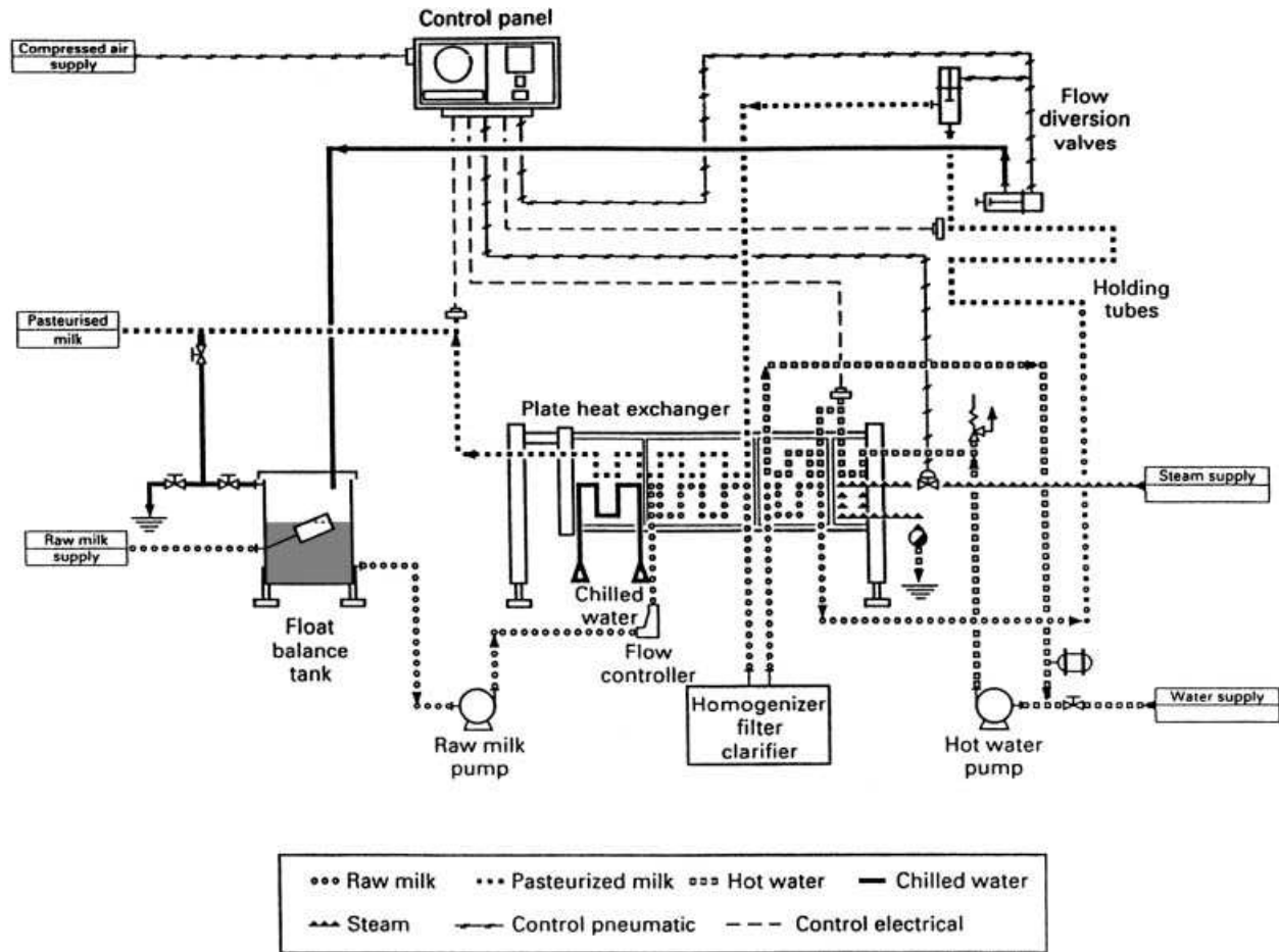
Fig. 2.6 Typical milk pasteurisation system; from [17] with permission.
