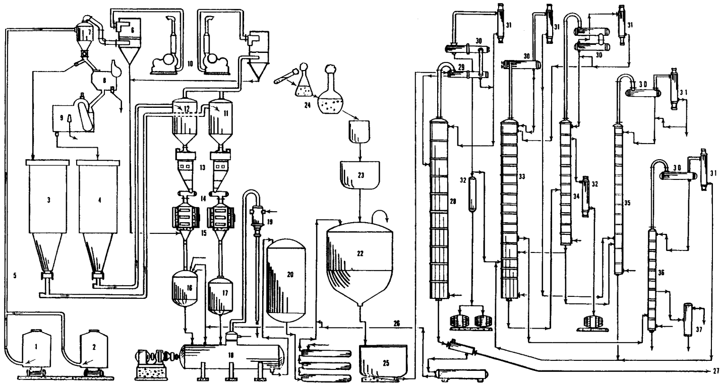
Fig. 14.20 Material process flow, modern beverage spirits plant; from [42] with permission. 1 cereal grains; 2 malt; 3 malt bin; 4 cereal grain bin; 5 unloading elevator; 6 dust filter; 7 collector; 8 scalperator; 9 millerator; 10 reclaiming exhaustor; 11 malt receiver; 12 cereal grain receiver; 13 automatic scale; 14 mill feeder; 15 roller mills; 16 precooker; 17 malt infusion; 18 cooker; 19 barometric condenser; 20 converter; 21 mash coolers; 22 fermenter; 23 final yeast propagator; 24 yeast culture and intermediate yeast propagator; 25 fermented-mash holding vessel; 26 stillage return system; 27 stillage flow to recovery system; 28 whisky separating column; 29 heat exchanger; 30 dephlegamator; 31 vent condenser; 32 product cooler; 33 selective distillation column; 34 product concentrating column; 35 aldehyde concentrating column; 36 fusel oil concentrating column; 37 fusel oil decanter.
