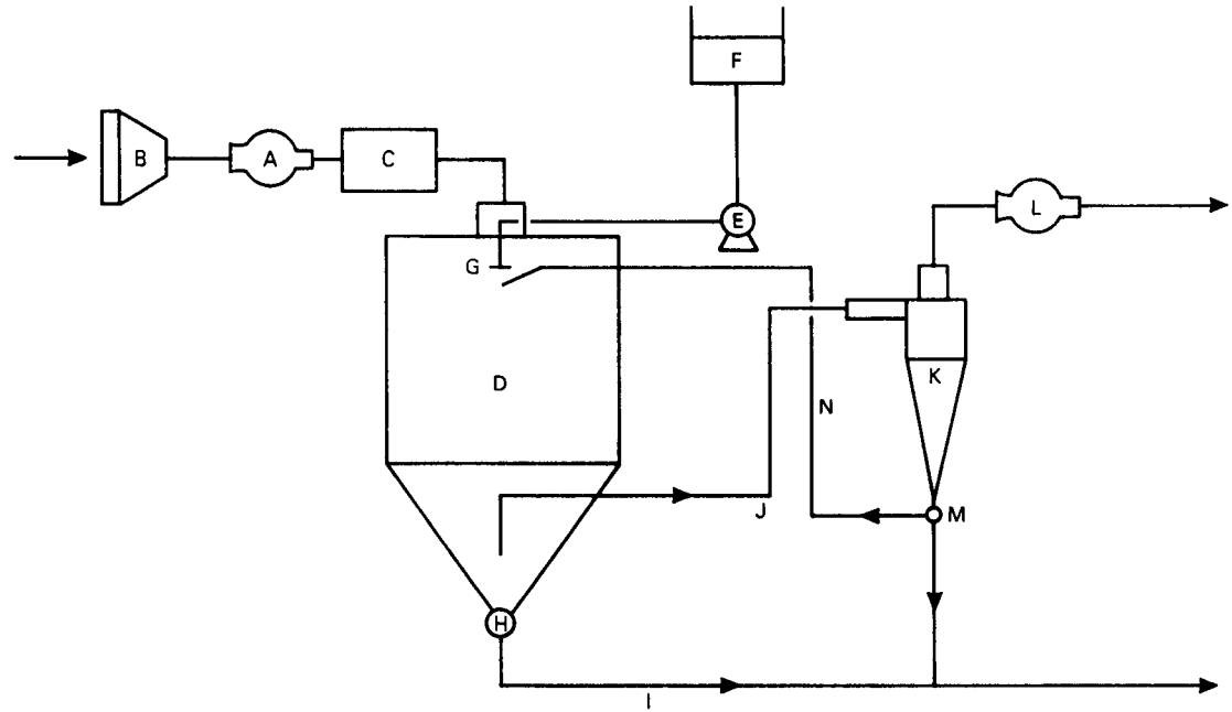
Fig. 3.11 Single-stage spray drying system; from [26] with permission.
