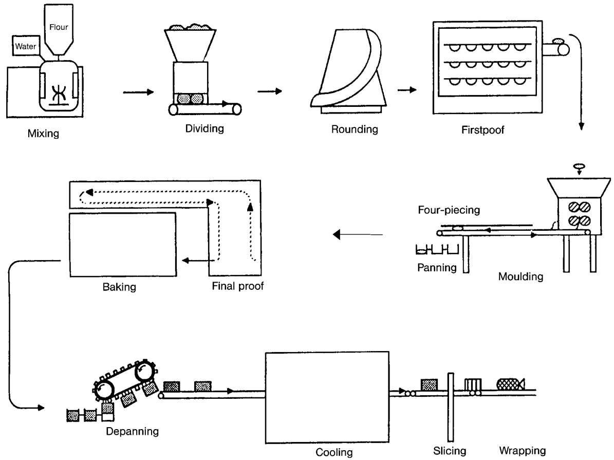
Fig. 8.2 The Chorleywood bread process [4].
