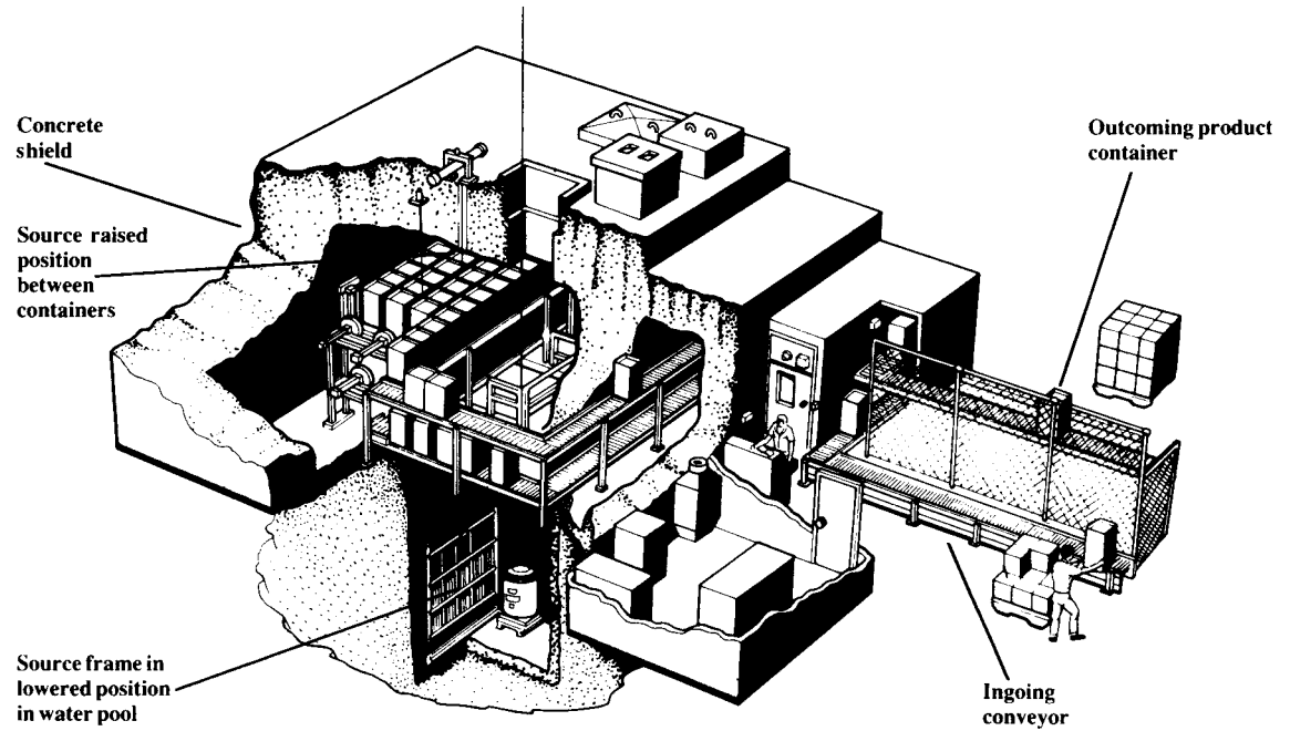
Fig. 5.4 Commercial automatic tote box \gamma ( ^{60}\text{Co} ) irradiator; by courtesy of Atomic Energy of Canada Ltd.
