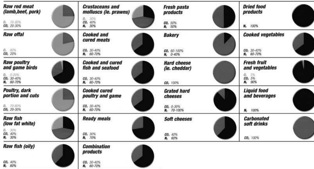
Fig. 9.12 Gas compositions commonly used in MAP food containers; by courtesy of Air Products.
