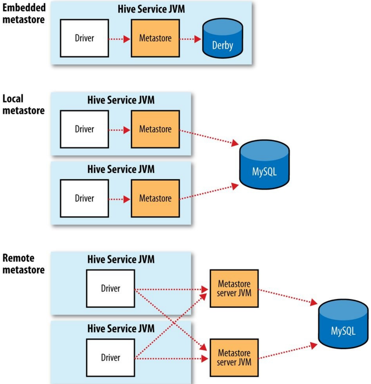
Figure 17-2. Metastore configurations
