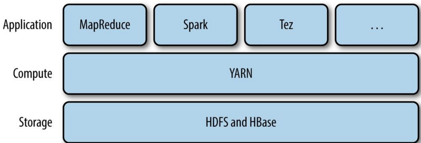
Figure 4-1. YARN applications
