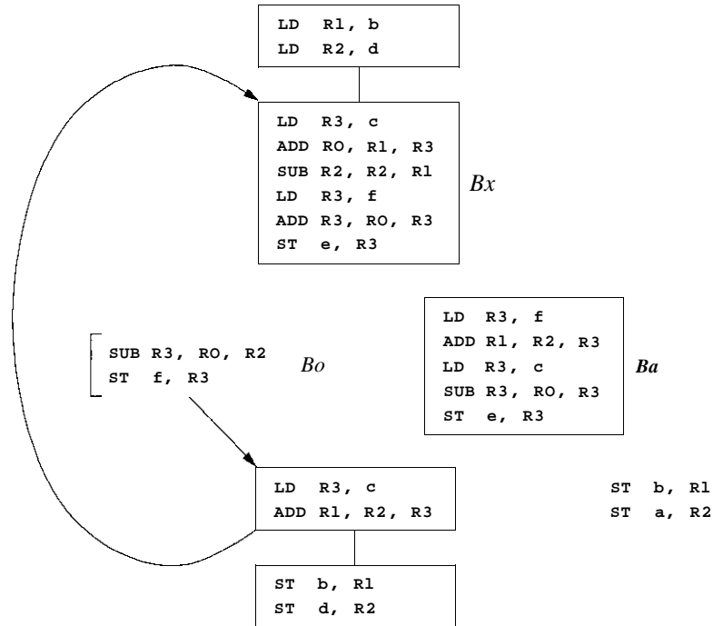
Figure 8.18: Code sequence using global register assignment
