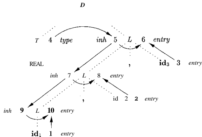
Figure 5.9: Dependency graph for a declaration float idi, id, id ,
