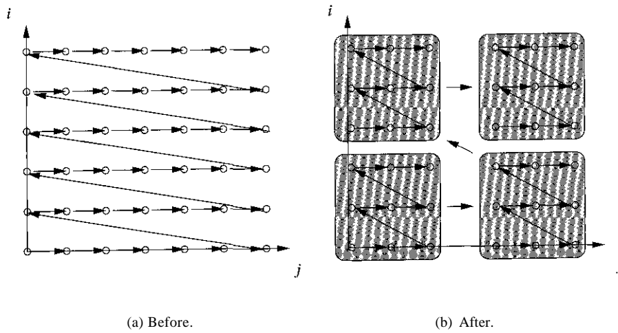
Figure 11.56: Execution order before and after blocking a 2-deep loop nest.
