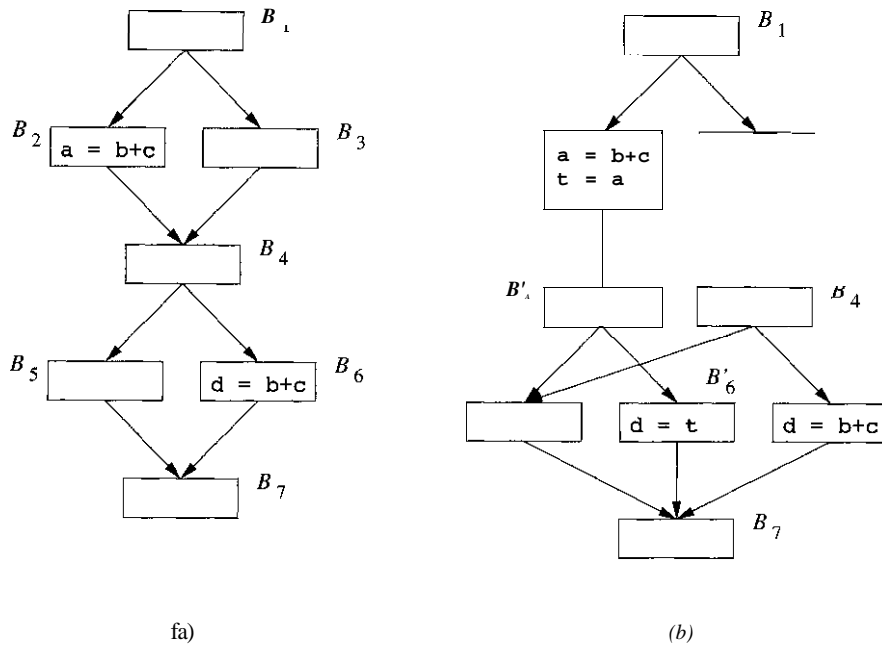
Figure 9.32: Code duplication to eliminate redundancies
