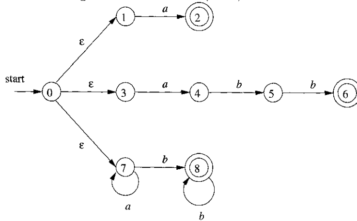
Figure 3.52: Combined NFA
