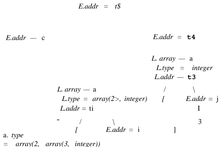
Figure 6.23: Annotated parse tree for c + a[i][j]
