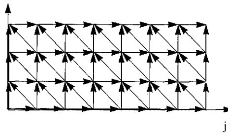
(b) Data dependences in the code.
