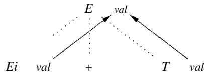
Figure 5.6: E.val is synthesized from E_i.val and E_i.val
