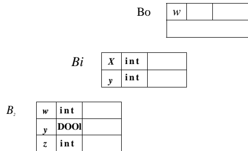
Figure 2.36: Chained symbol tables for Example 2.15
