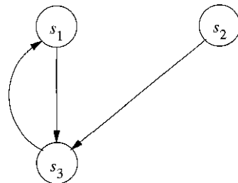
(b) Its dependence graph.
