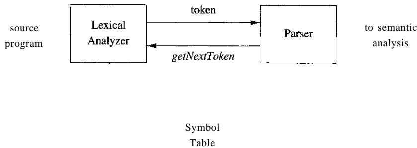
Figure 3.1: Interactions between the lexical analyzer and the parser
