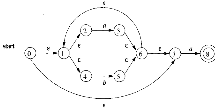
Figure 3.46: NFA for rr
