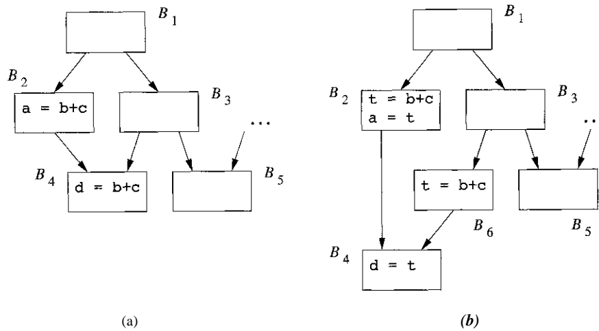
Figure 9.31: B_3 \rightarrow B_4 is a critical edge
