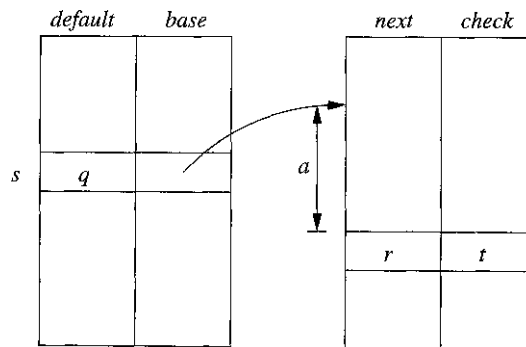
Figure 3.66: Data structure for representing transition tables
