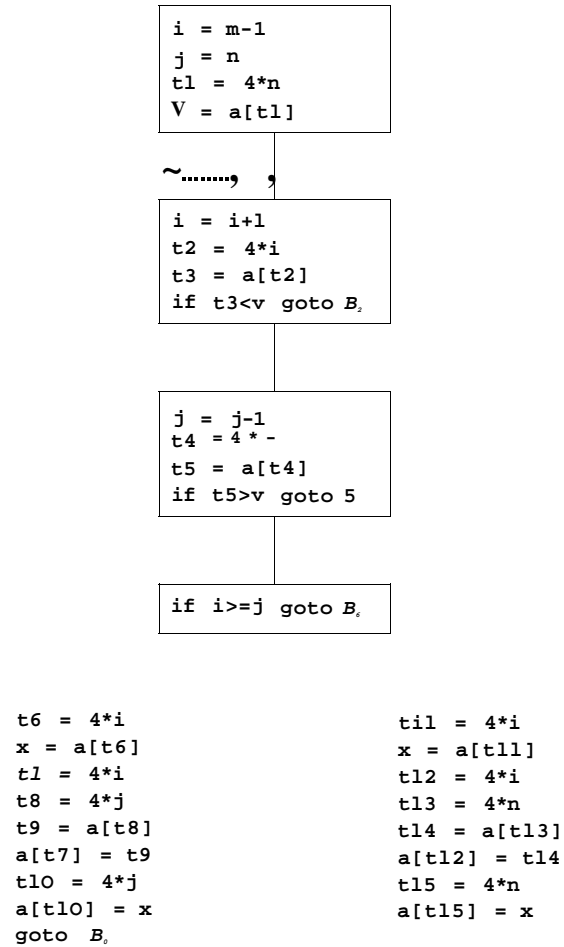
Figure 9.3: Flow graph for the quicksort fragment
