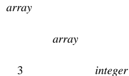
Figure 6.14: Type expression for int [2] [3]
