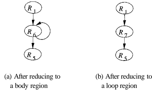
Figure 9.49: Steps in the reduction of the flow graph of Fig. 9.47 to a single region
