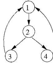
Figure 9.46: Two loops with the same header
