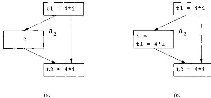
Figure 9.17: Potential common subexpressions across blocks
