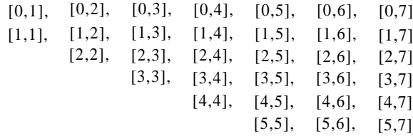
Figure 11.12: Iteration order for loop nest of Fig. 11.10
