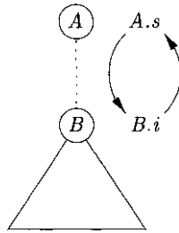
Figure 5.2: The circular dependency of A.s and BA on one another
