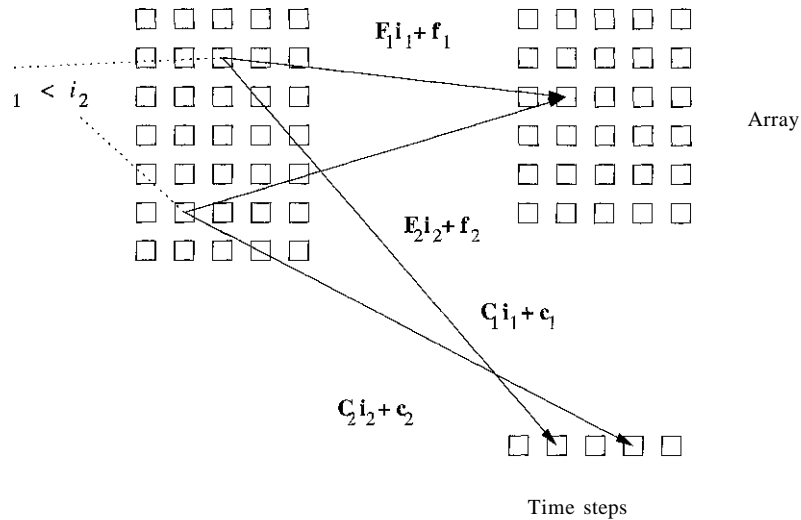
Figure 11.54: Time-Partition Constraints
