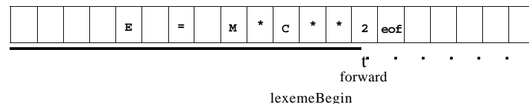
Figure 3.3: Using a pair of input buffers
