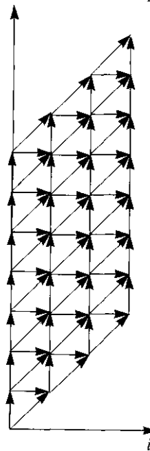
Figure 11.51: Fully permutable version of the code Fig. 11.50
