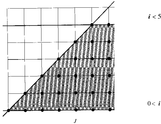
Figure 11.11: The iteration space of Example 11.6
