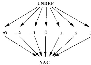
Figure 9.25: Semilattice representing the possible "values" of a single integer variable
