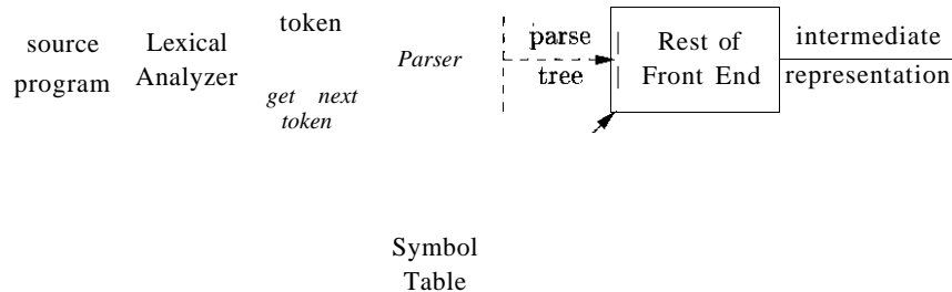
Figure 4.1: Position of parser in compiler model
