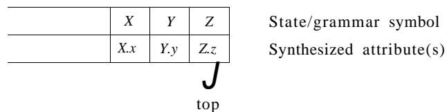
Figure 5.19: Parser stack with a field for synthesized attributes
