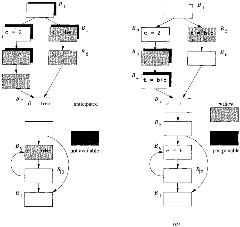
Figure 9.33: Flow graph of Example 9.30
