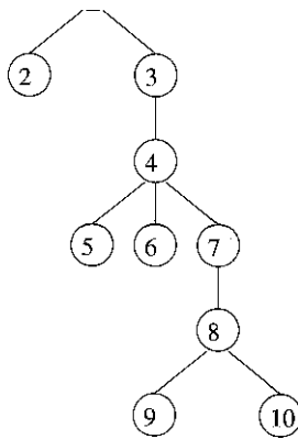
Figure 9.39: Dominator tree for flow graph of Fig. 9.38
