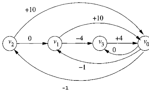
Figure 11.21: Graph for the constraints of Example 11.37
