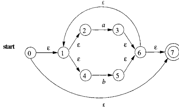
Figure 3.45: NFA for r_1
