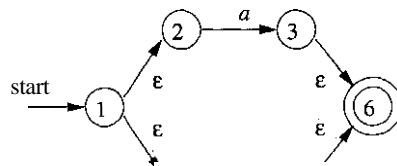
Figure 3.44: NFA for r_1
