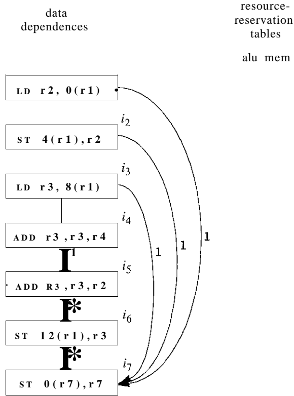
Figure 10.7: Data-dependence graph for Example 10.6
