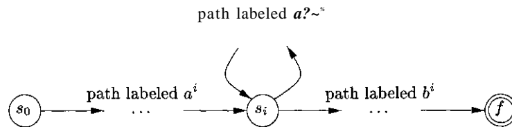
Figure 4.6: DFA D accepting both a^i b^i and a^i b^i .
