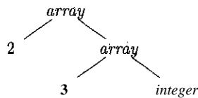
Figure 5.15: Type expression for int[2][3]
