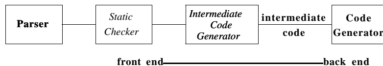
Figure 6.1: Logical structure of a compiler front end
