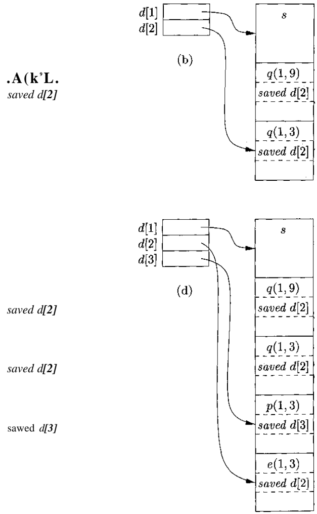
Figure 7.14: Maintaining the display
