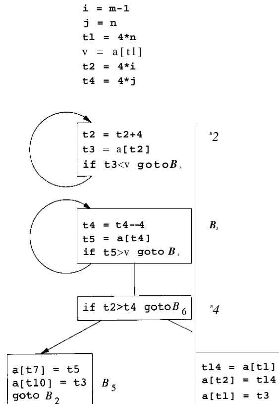
Figure 9.9: Flow graph after induction-variable elimination
