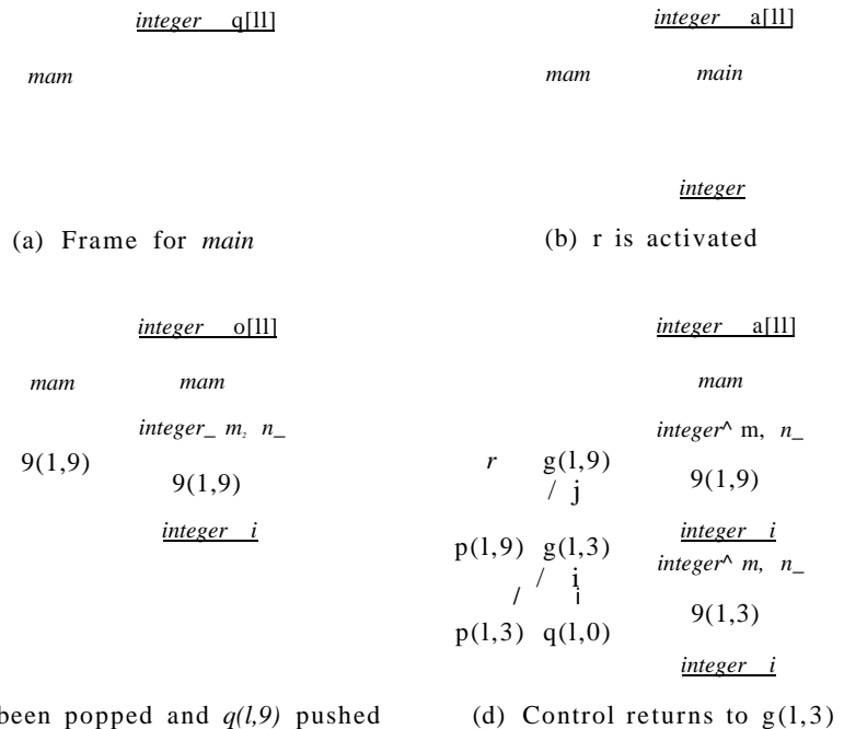
Figure 7.6: Downward-growing stack of activation records
