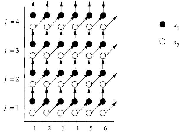
Figure 11.27: Dependences of the code in Example 11.41
