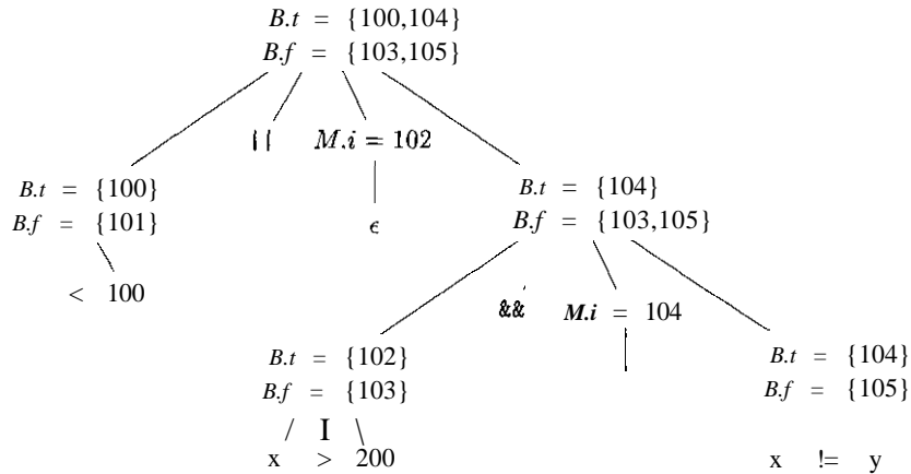
Figure 6.44: Annotated parse tree for x < 100 \text{ I I } x > 200 \text{ kk } x \neq y
