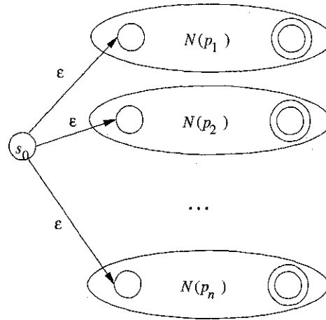
Figure 3.50: An NFA constructed from a Lex program
