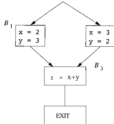
Figure 9.27: An example demonstrating that the constant propagation framework is not distributive
