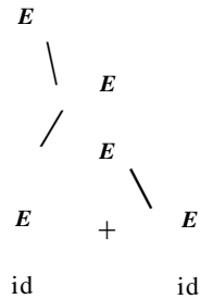
Figure 4.3: Parse tree for -(id + id)
