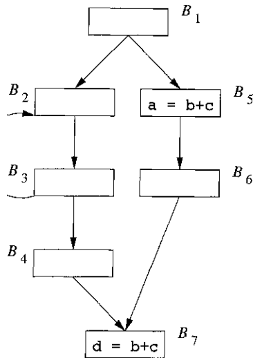
Figure 9.36: Flow graph for Example 9.33 to illustrate the need for postponing an expression
