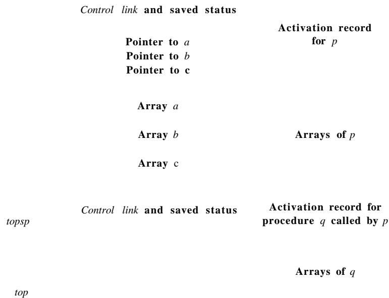
Figure 7.8: Access to dynamically allocated arrays
