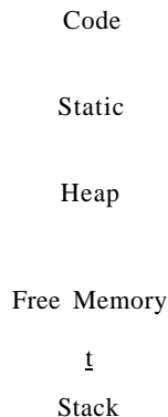
Figure 7.1: Typical subdivision of run-time memory into code and data areas
