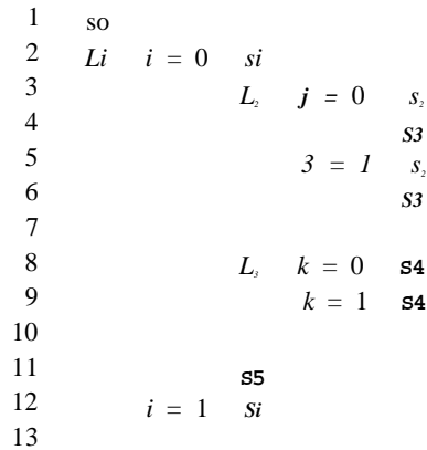
Figure 11.45: Execution order of the program in Example 11.53.
