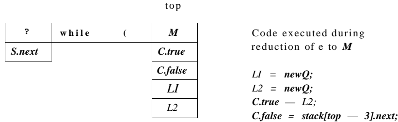
Figure 5.36: LR parsing stack after reduction of e to M
