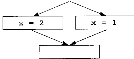
Figure 10.14: Example illustrating the change in data dependences due to code motion.
