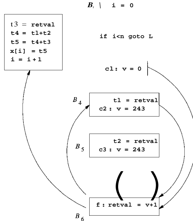
Figure 12.4: The control-flow graph for Fig. 12.3, treating function calls as control flow
