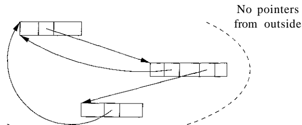
Figure 7.18: An unreachable, cyclic data structure
