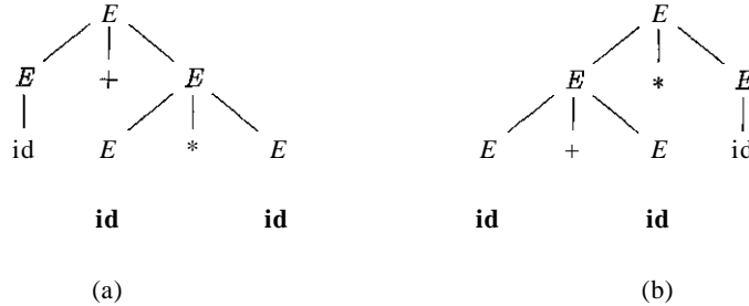
Figure 4.5: Two parse trees for \text{id+id*id}
