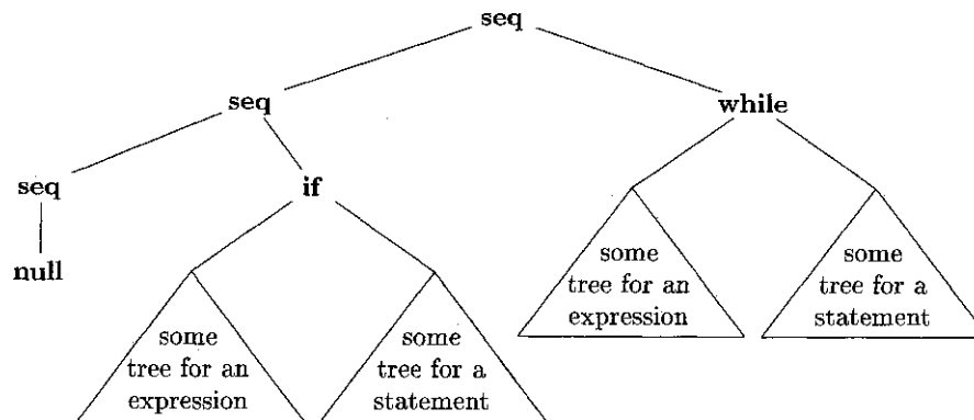
Figure 2.40: Part of a syntax tree for a statement list consisting of an if-statement and a while-statement
