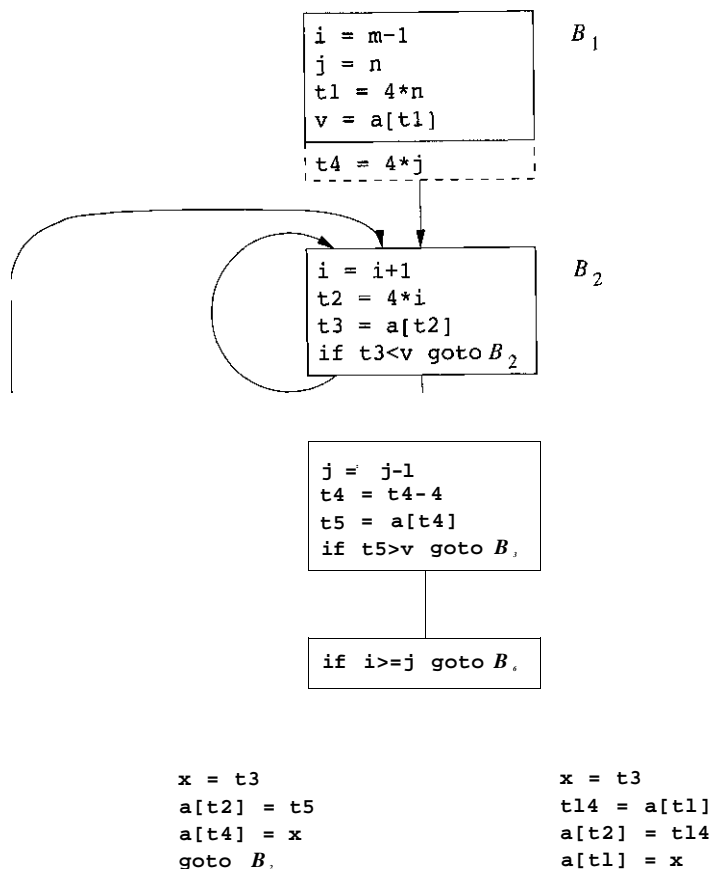
Figure 9.8: Strength reduction applied to 4 * j in block S_3
