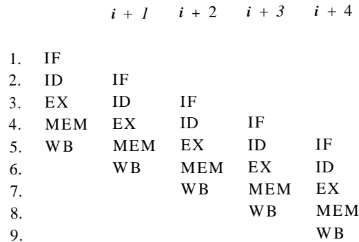
Figure 10.1: Five consecutive instructions in a 5-stage instruction pipeline
