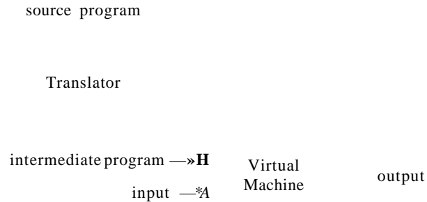
Figure 1.4: A hybrid compiler
