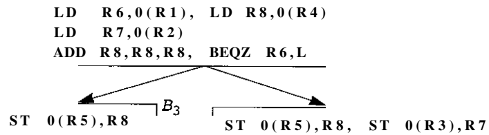
(c) Globally scheduled machine code
