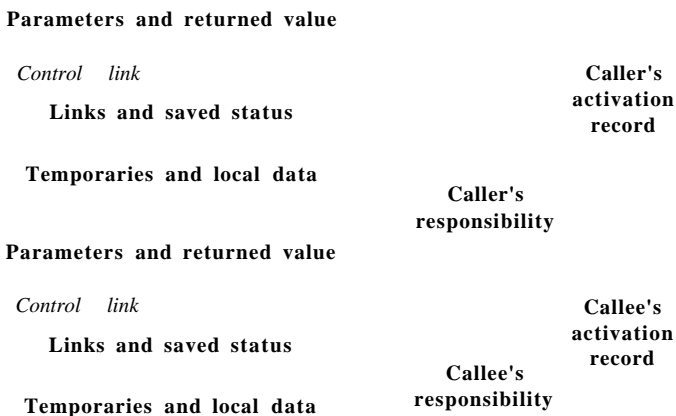
Figure 7.7: Division of tasks between caller and callee
