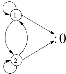
Figure 3.61: Directed graph for the function followpos
