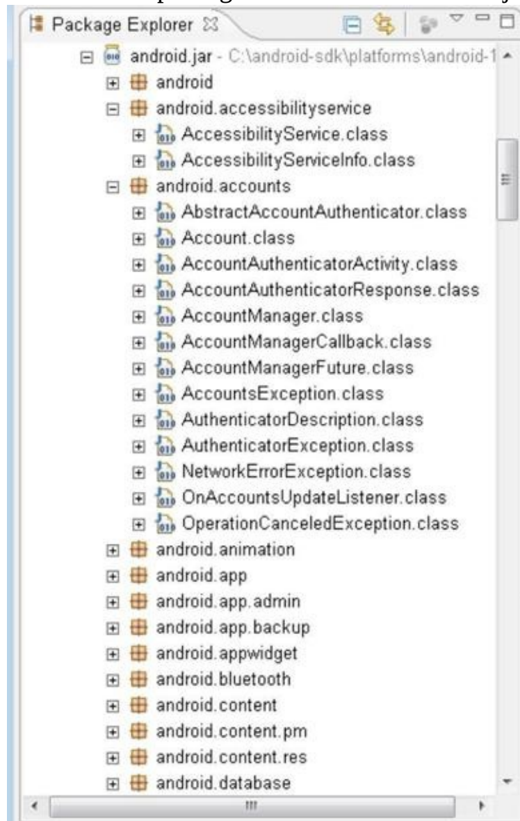
Figure 3-17: Some of the packages and classes in android.jar .
