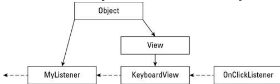
Figure 4-1: The interface hierarchy cuts across the class hierarchy.
