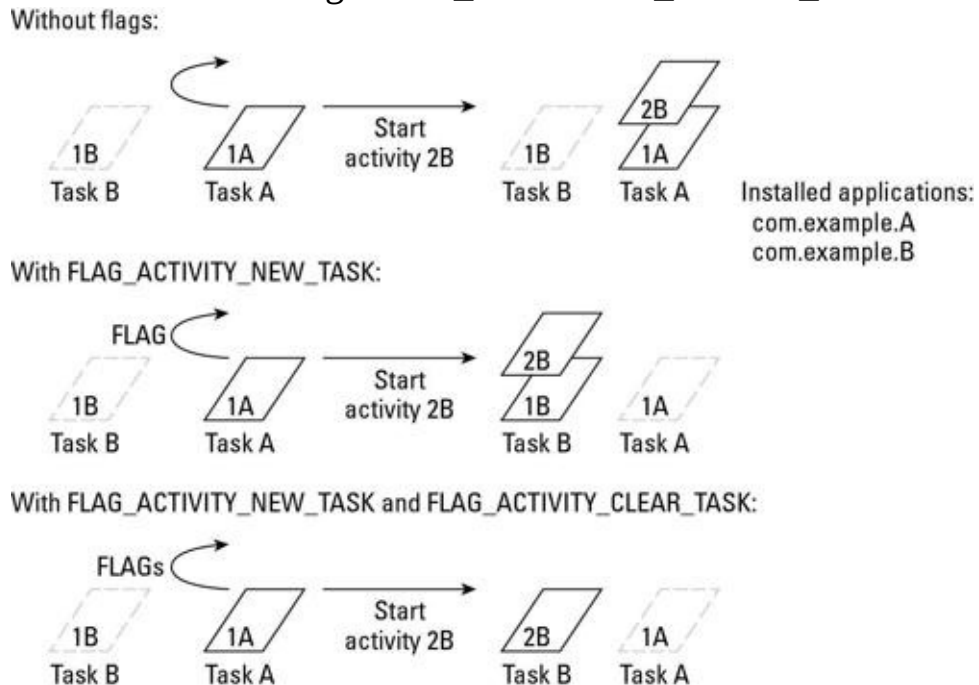
Figure 2-18: The effect of adding FLAG_ACTIVITY_CLEAR_TASK .
