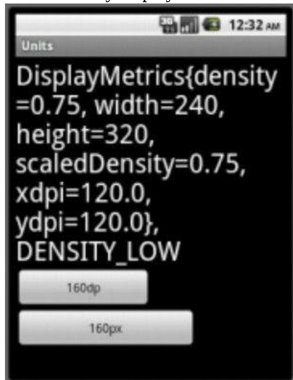
Figure 1-4: A low-density display.
