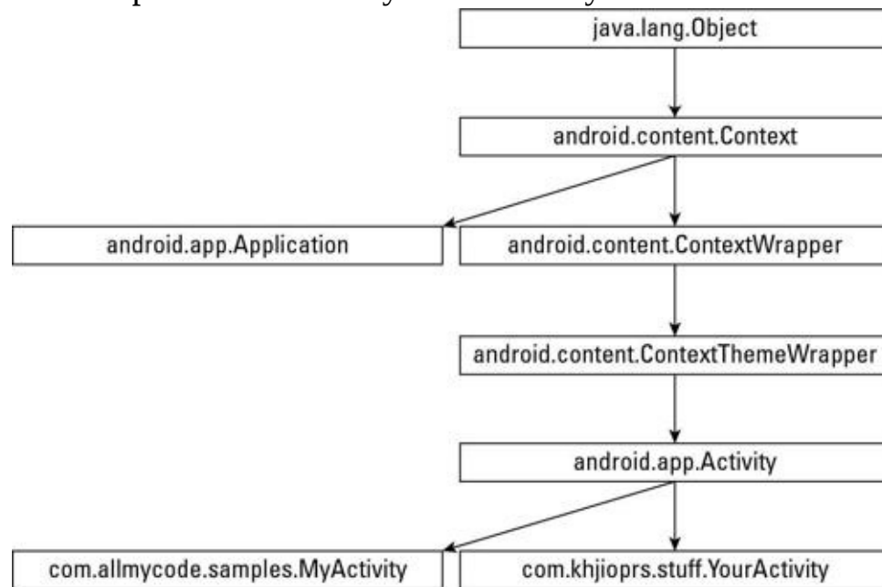
Figure 2-4: A small part of the Activity class's family tree.
