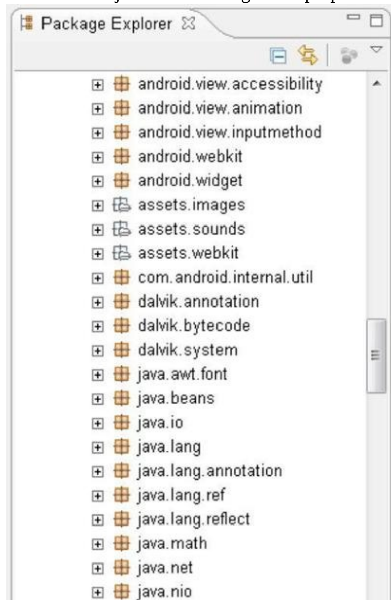
Figure 3-18: The android.jar file includes general-purpose Java packages.
