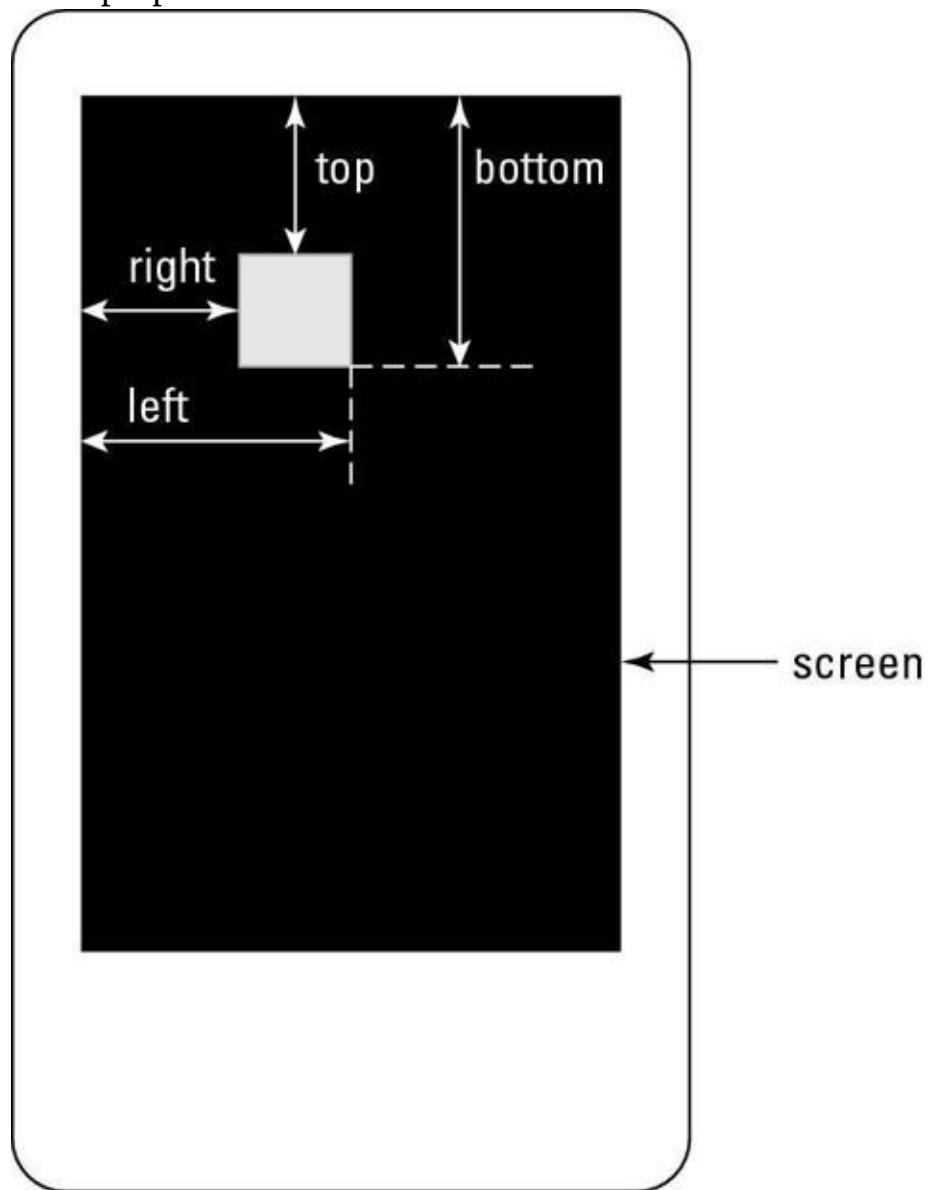
Figure 3-11: The properties of a Rect instance.
