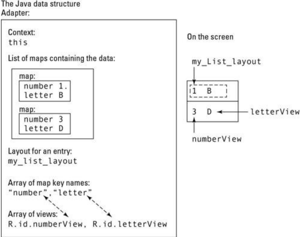
Figure 2-13: An adapter for the list in this section’s code.
