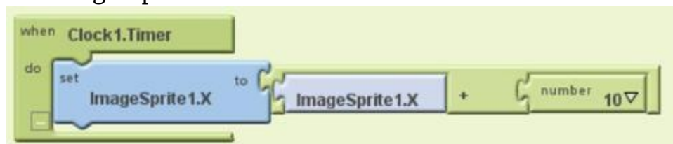
Figure 2-10: Moving a sprite . . . one click at a time.
