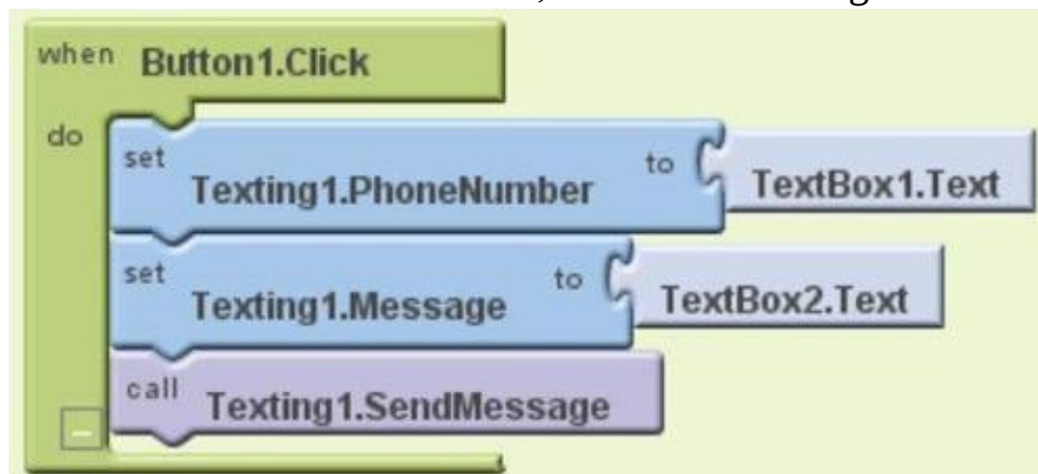
Figure 2-5: When the user clicks the button, send a text message.
