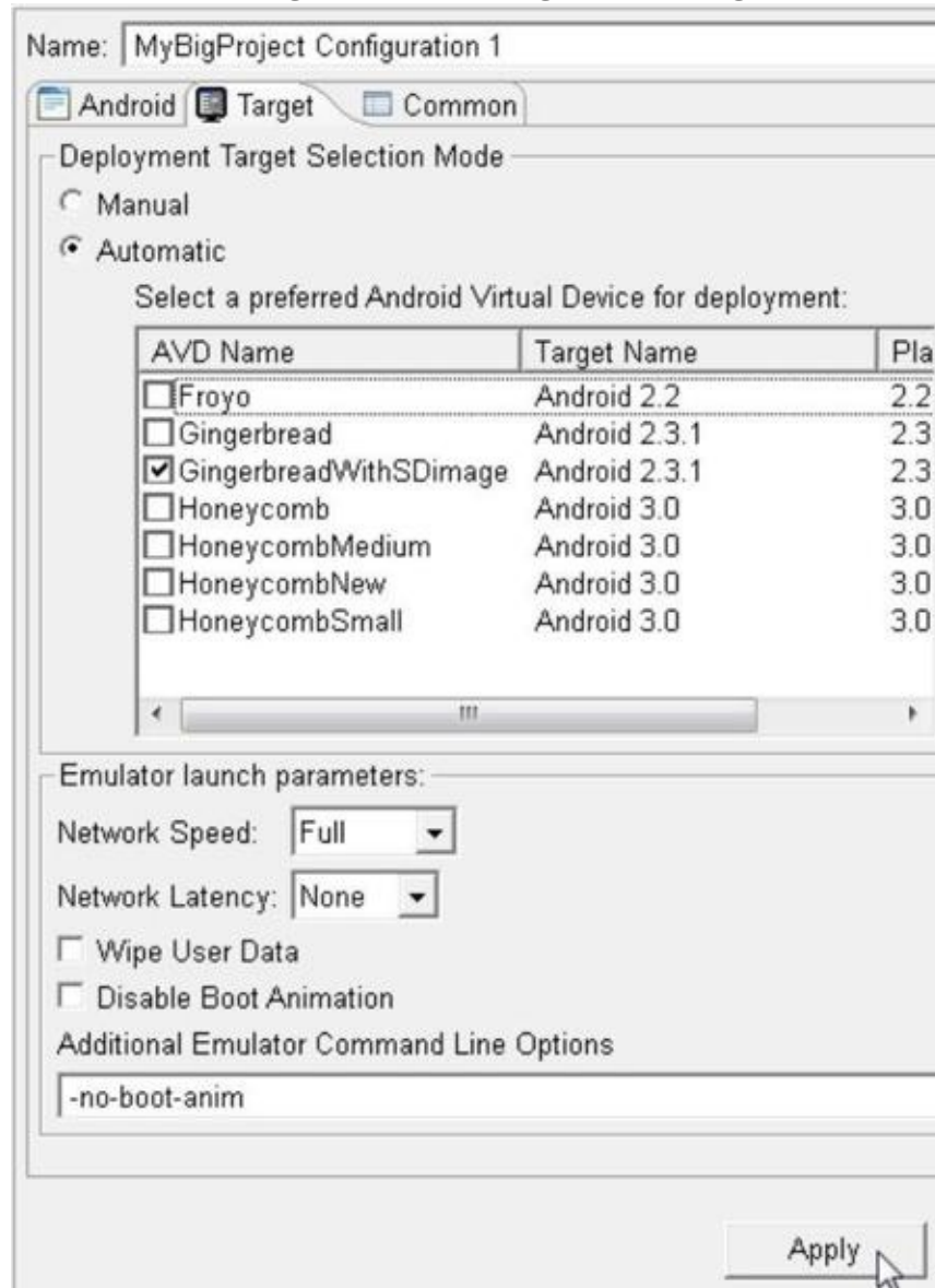
Figure 1-29: The Run Configurations dialog box's Target tab.
