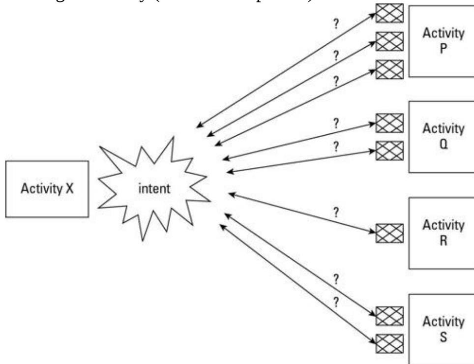
Figure 2-1: Finding an activity (or other component) to match an intent.
