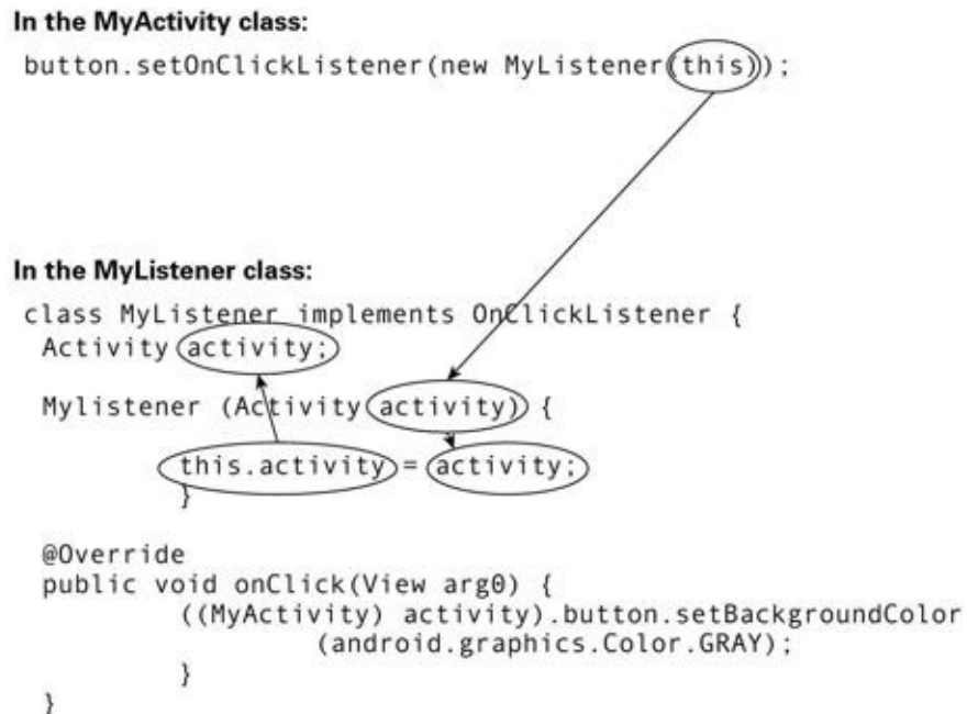
Figure 4-3: How a listener remembers its creator.
