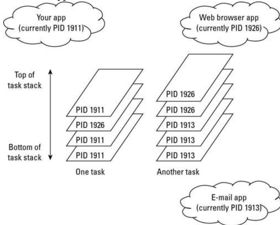
Figure 1-1: Activities, apps, and tasks.
