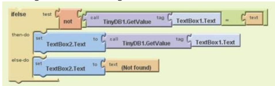
Figure 2-17: Failing to find, but failing with a flourish.
