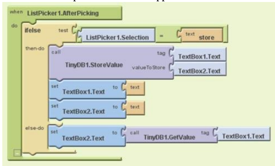
Figure 2-16: Blocks for simple control of an App Inventor database.
