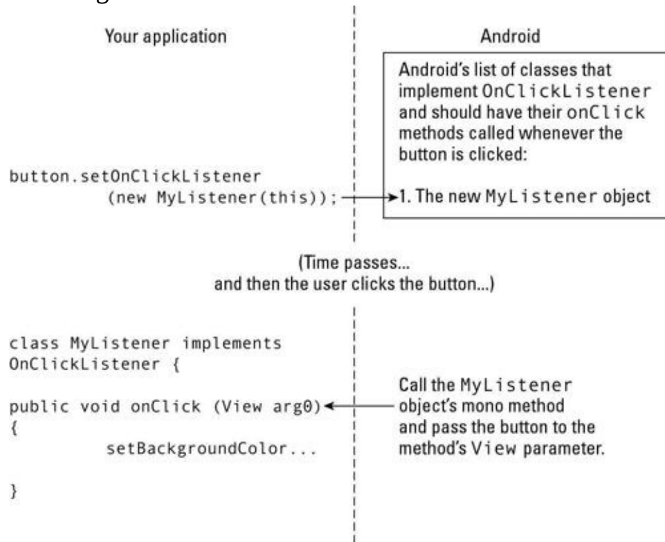
Figure 4-2: Handling an event.
