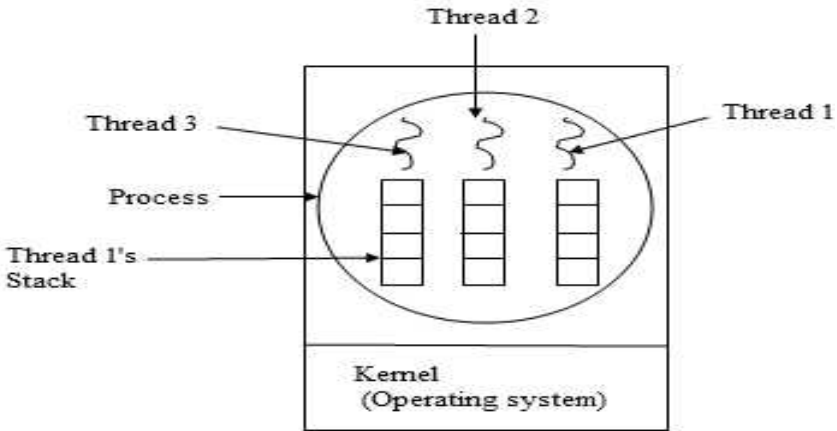
Fig 2.5: Threads
