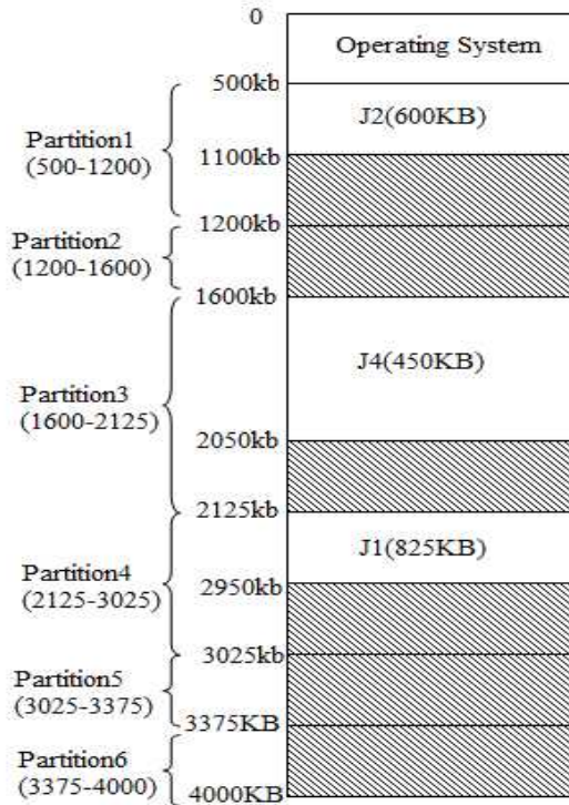
Fig.3.12: Memory allocation
