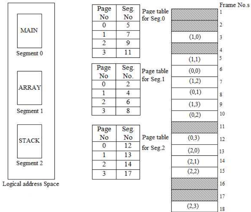
Fig.3.23: Paged Segmentation
