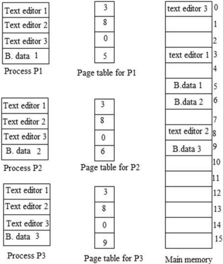
Fig.3.18: Shared Paging
