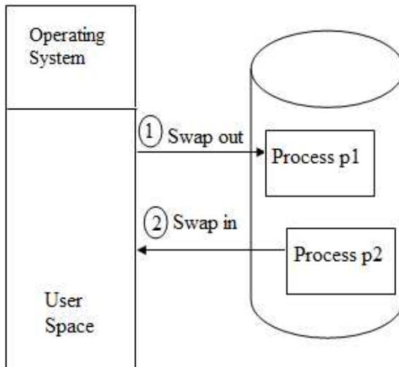
Fig.3.7: Swapping
